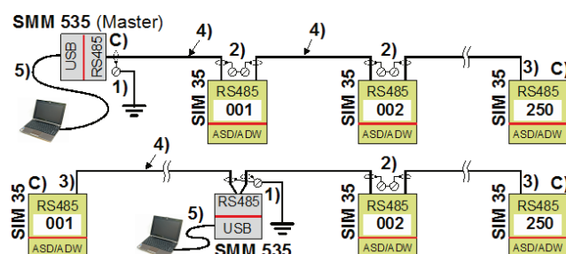
Fig. 4 Design of the ASD network
